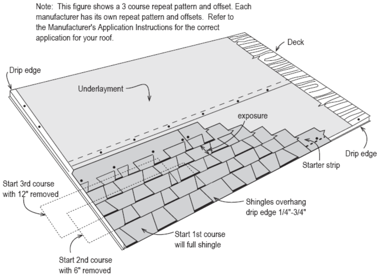
Figure 2: Asphalt Shingle roofing system installation detail
