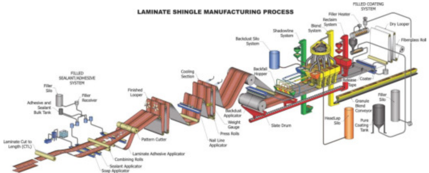
Figure 1: Laminated shingle production diagram
